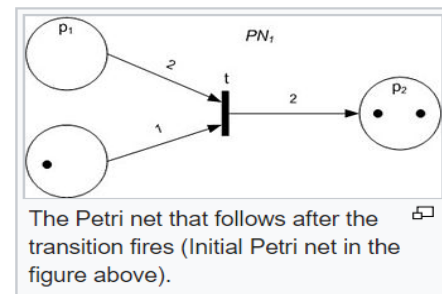
Figure 1: Petri Net [2]
