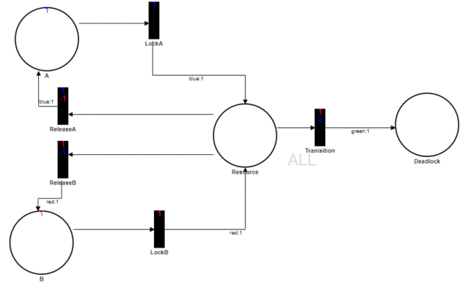
Figure 3: Colored Petri Net DSM
