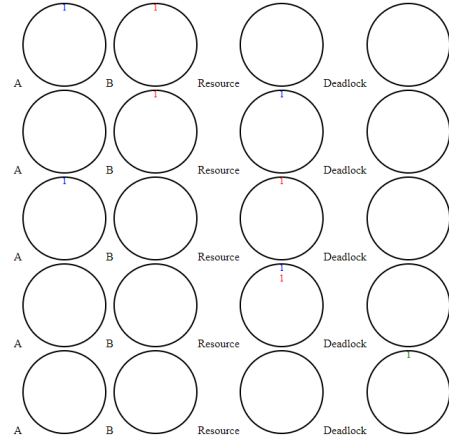
Figure 9: Results of the AllPossible Plugin
