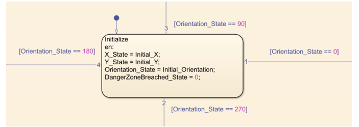
Figure 7: Initialize Mode For Flight Controller
