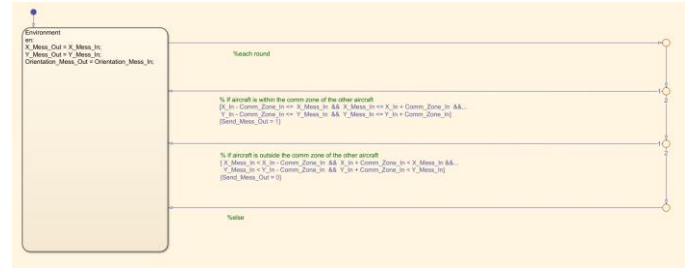
Figure 13: Aircraft Communications Environment
