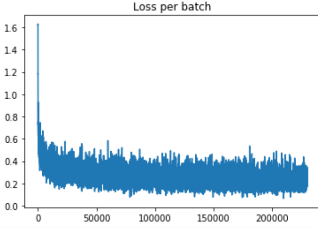
Fig. 9: Trial 1
