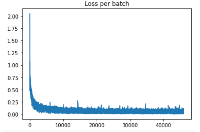
Fig. 12: Trial 4
