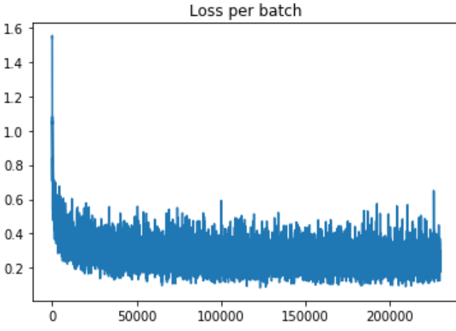
Fig. 10: Trial 2
