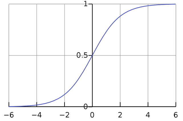
Fig. 6: Sigmoid Curve [6]
