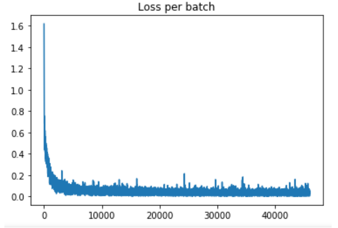
Fig. 13: Trial 5
