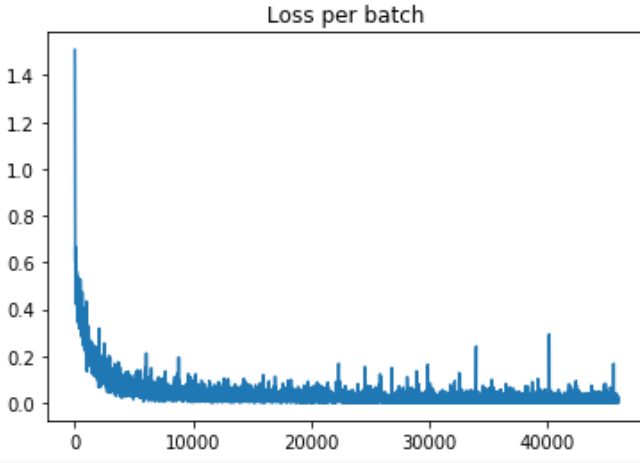
Fig. 11: Trial 3
