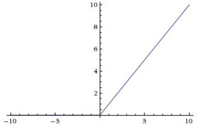
Fig. 7: ReLU Curve [7]
